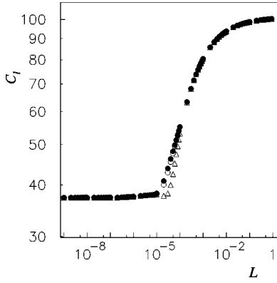
FIG. 11. Contour length C_l of the average configuration as a function of L for N=100 , K=10 , and \theta_0=\pi/180 ( \bullet ), \theta_0=\pi/3 ( \circ ), and \theta_0=2\pi/3 ( \triangle ).
