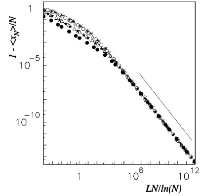
FIG. 6. Average extension \langle x_N \rangle of the chain in the direction of the force field as a function of the field strength L . The symbols correspond to the same parameters as in Fig. 5. The straight line has slope -1 .
