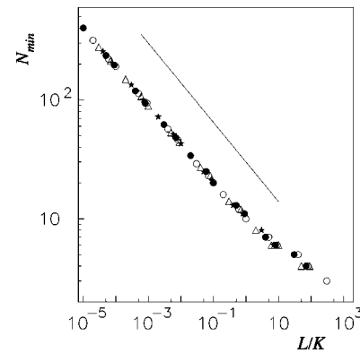
FIG. 3. N_{\min} as a function of L/K for K=1 (●), K=10 (○), K=100 (△), K=1000 (★). The straight line has slope -1/3 .
