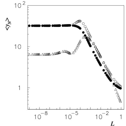
FIG. 10. Average transverse extension \langle y_N \rangle as a function of L for N=100 , K=10 , and \theta_0 = \pi/3 (●), \theta_0 = 2\pi/3 (O), and \theta_0 = 17\pi/18 ( \Delta ).
