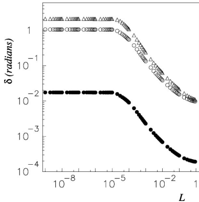
FIG. 12. Angle \delta between a line through the end points of the chain and the direction of the force field as a function of L for N=100 , K=10 , and \theta_0=\pi/180 ( \bullet ), \theta_0=\pi/3 ( \circ ), and \theta_0=2\pi/3 ( \triangle ).
