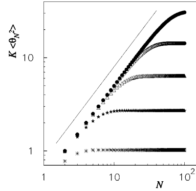
FIG. 2. Average angular fluctuations K\langle\theta_N^2\rangle of the final chain segment as a function of N for L/K=10^{-5} (●), L/K=10^{-4} (○), L/K=10^{-3} (△), L/K=10^{-2} (★), L/K=10^{-1} (*). The straight line has slope 1.
