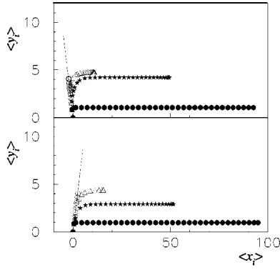
FIG. 7. Average positions \langle x_i \rangle, \langle y_i \rangle of a chain of length N = 100 with K=1 , \theta_0 = \pi/3 (lower panel), and \theta_0 = 2\pi/3 (upper panel), with L=10^{-5} (O), L=10^{-4} ( \Delta ), L=10^{-3} (★), and L=10^{-1} (●). The straight line indicates the tilt angle \theta_0 .
