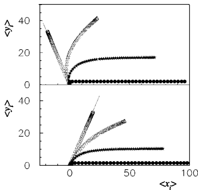
FIG. 8. Average positions \langle x_i \rangle, \langle y_i \rangle of a chain of length N = 100 with K=10 , \theta_0 = \pi/3 (lower panel), and \theta_0 = 2\pi/3 (upper panel), with L=10^{-5} (O), L=10^{-4} ( \Delta ), L=10^{-3} (★), and L=10^{-1} (●). The straight line indicates the tilt angle \theta_0 .
