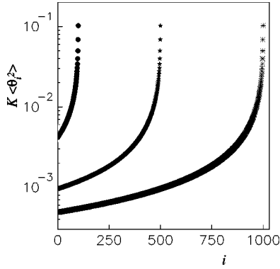
FIG. 1. Average angular fluctuations K\langle\theta_i^2\rangle for L/K=0.1 and N=100 (●), N=500 (★), N=1000 (*).
