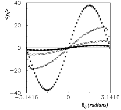
FIG. 9. Average transverse extension \langle y_N \rangle as a function of \theta_0 for N=100 , K=10 , and L=10^{-9} (*), L=10^{-5} (★), L=10^{-3} ( \Delta ), L=10^{-2} (O), L=10^{-1} (●).
