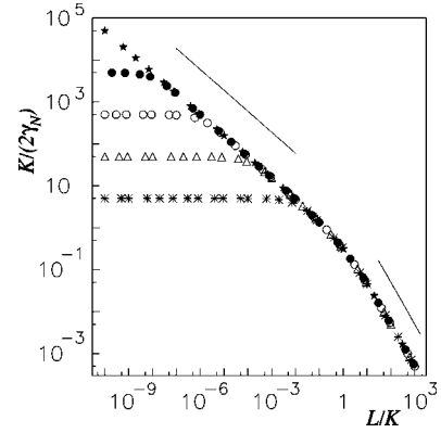
FIG. 13. K\langle\theta_N^2\rangle=K/(2\gamma_N) for a polymer pulled at the ends as a function of L/K for N=10 ( * ), N=100 ( \triangle ), N=1000 ( \circ ), and N=10\,000 ( \bullet ), together with the exact result (42) for N\rightarrow\infty ( * ). The straight lines have slopes -1/2 and -1 , respectively.
