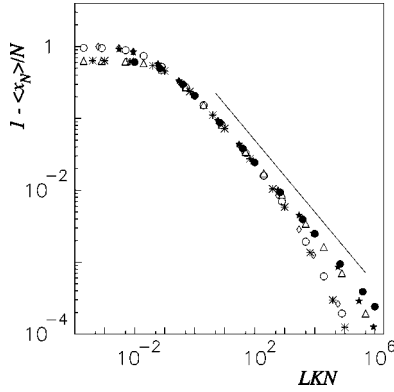
FIG. 5. Average extension \langle x_N \rangle of the chain in the direction of the force field as a function of the field strength L , for K=10 , N=100 (*); K=10 , N=1000 ( \circ ); K=10 , N=10000 ( \diamond ); K=100 , N=1000 ( \triangle ); K=100 , N=10000 ( \star ); K=1000 , N=10000 ( \bullet ). The straight line has slope -1/2 .
