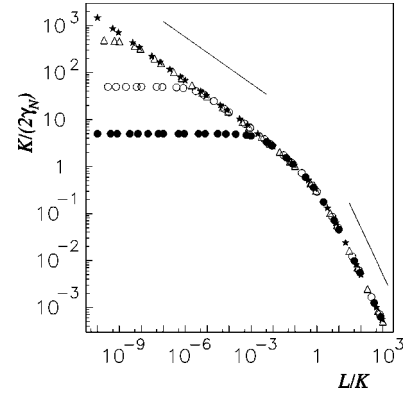
FIG. 4. K\langle \theta_N^2 \rangle = K/(2\gamma_N) for a polymer in a constant force field as a function of L/K for N=10 ( \bullet ), N=100 ( \circ ), and N=1000 ( \triangle ), together with the exact result (28) for N \rightarrow \infty ( \star ). The straight lines have slopes -1/3 and -1 , respectively.
