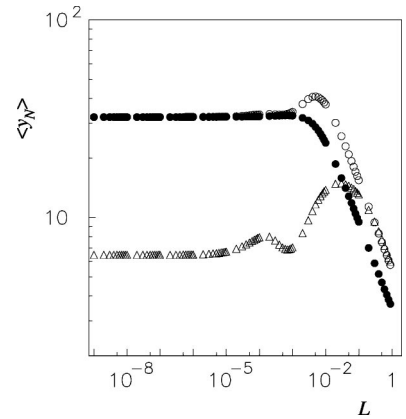
FIG. 14. Average transverse extension \langle y_N \rangle of a polymer pulled at its ends as a function of L for N=100 , K=10 , and \theta_0=\pi/3 ( \bullet ), \theta_0=2\pi/3 ( \circ ), \theta_0=17\pi/18 ( \triangle ).
